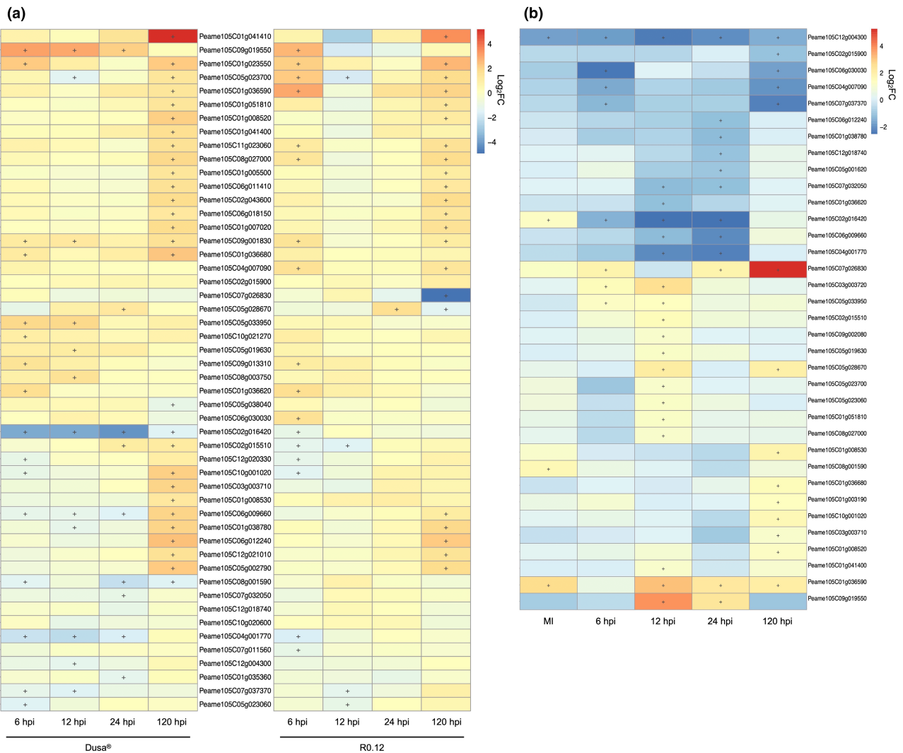
FIGURE 5 Expression level differences of WRKY genes in two avocado rootstocks following Phytophthora cinnamomi inoculation. (a) Heatmap of the differences in expression levels as \log_2 -fold-change ( \log_2FC ) in Dusa (partially resistant) and R0.12 (susceptible) rootstocks at different time points (hours post-inoculation; hpi) following inoculation. Mock-inoculated samples are set as the reference, thus positive \log_2FC values (red) indicate higher expression levels in inoculated samples, and negative \log_2FC values (blue) indicate lower expression levels in inoculated samples. (b) Heatmap showing the level of WRKY expression compared between the two rootstocks, with R0.12 set as the reference. Positive \log_2FC values (red) indicate higher WRKY expression levels in Dusa and negative \log_2FC values (blue) indicate higher levels of expression in R0.12. (+ symbols indicate significance, \log_2FC \geq |1|, p \leq 0.05 ; MI, mock-inoculated).
